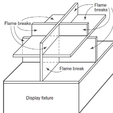
FIGURE A.7.10.3 Flame Break Design.
