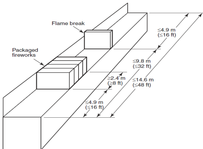
FIGURE A.7.10.3.4 Packaged Fireworks Merchandise and Flame Break Requirements.
